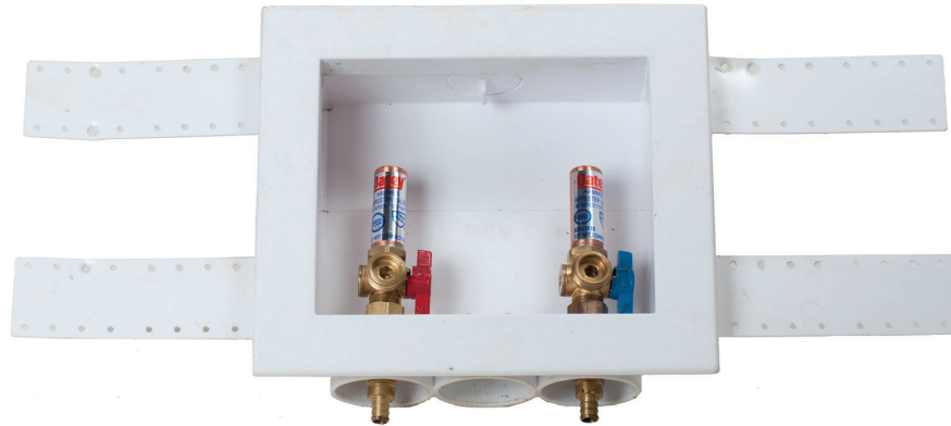
Figure 76 Laundry box. (Oatey, n.d.) Used with permission
