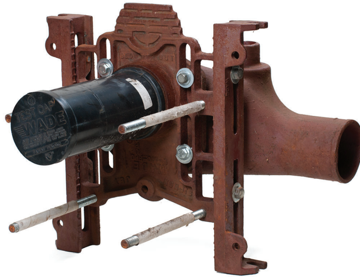
Figure 79 Horizontal, left-hand, siphon jet water-closet carrier. (Skilled Trades BC, 2021) Used with permission.
