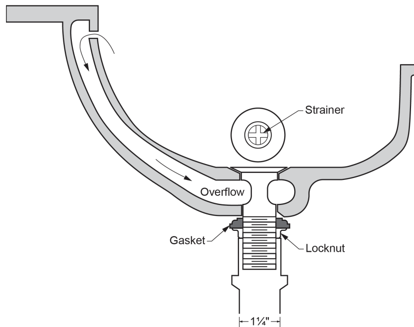
Figure 50 Basin patent overflow (PO) fitting. (Skilled Trades BC, 2021) Used with permission.
